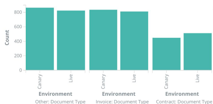
Testset Distribution
